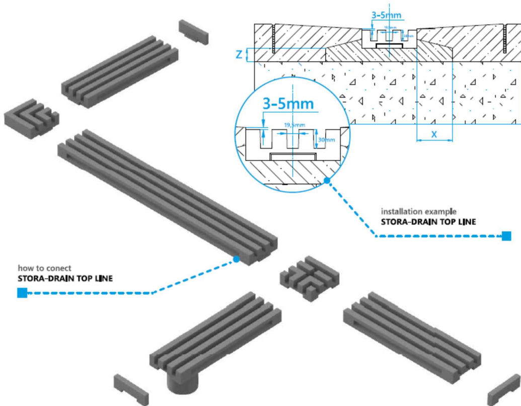
cross connection
